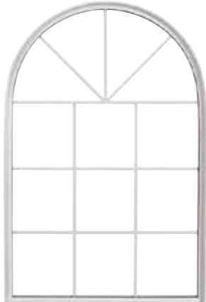
RADIUS/ARCH TOP Min 1'1" – Max 8'6" Structural Class HC-40 Not available at all locations
